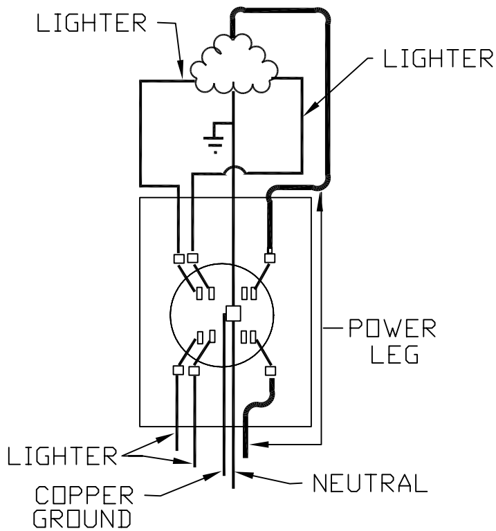
THREE PHASE 4 WIRE DELTA
