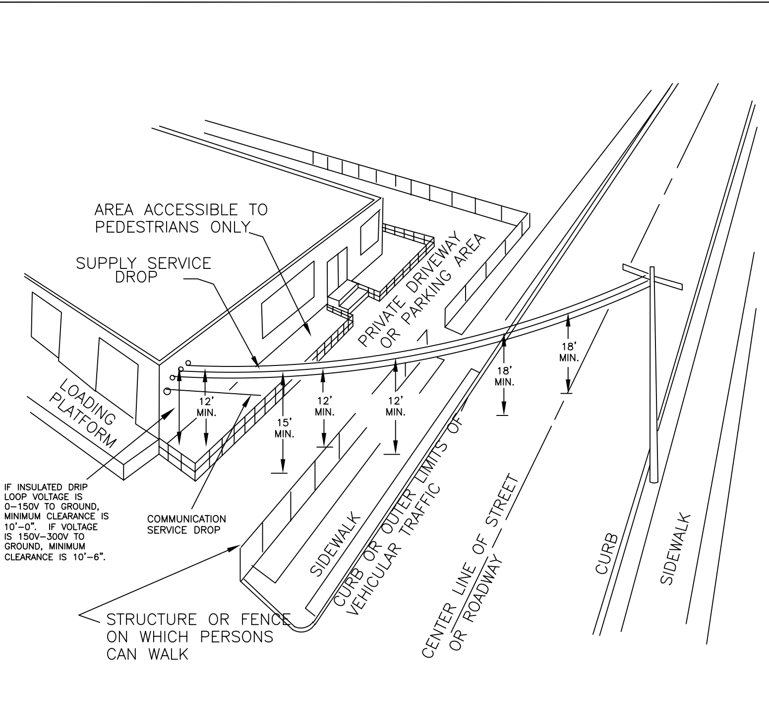
GROUND CLEARANCES FOR SUPPLY SERVICE DROPS INDUSTRIAL AND COMMERCIAL PREMISES
